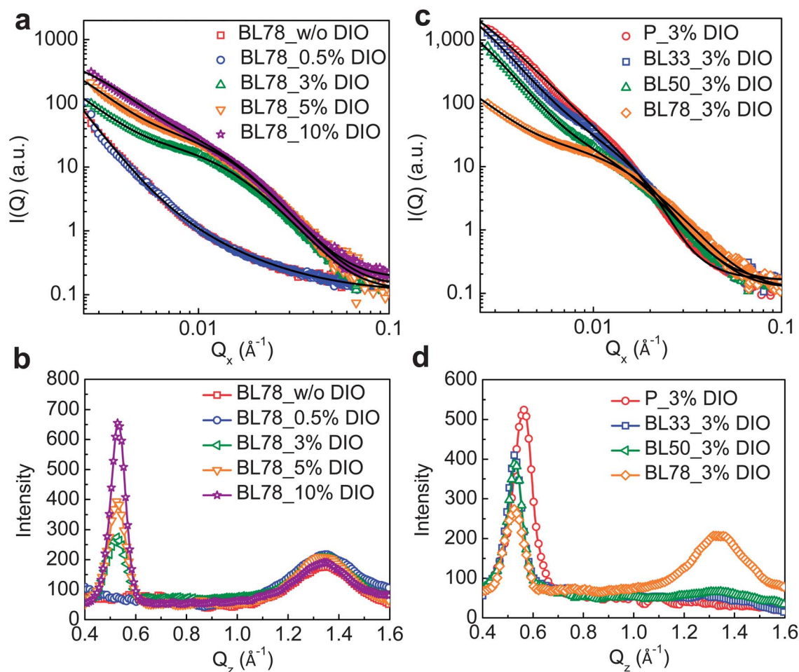
Fig. 2 (a) GISAXS and (b) GIWAXS profiles of PCPDTBT/PCBM (78 wt% PCBM) blend films processed without and with 0.5%, 3%, 5%, 10% DIO, i.e. BL78_w/o DIO, BL78_0.5% DIO, BL78_3% DIO, BL78_5% DIO, and BL78_10% DIO respectively. (c) GISAXS and (d) GIWAXS profiles of pristine PCPDTBT film and PCPDTBT/PCBM blend films with 33%, 50%, 78 wt% PCBM respectively. These films were processed with 3% DIO, i.e. P_3% DIO, BL33_3% DIO, BL50_3% DIO, and BL78_3% DIO. The solid lines in (a) and (c) represent the model-fitted intensities.
